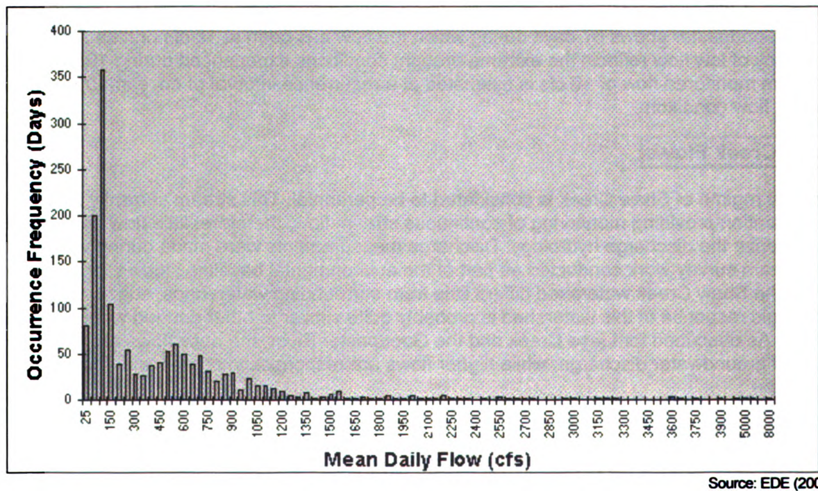
Figure 3.5-3 Goodpaster River Mean Daily Flow Frequency Distribution 1997-2001
