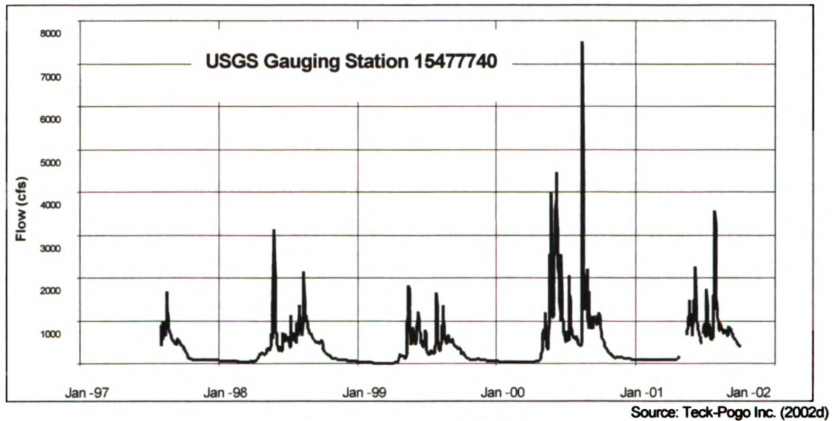
Figure 3.5-2 Goodpaster River Mean Daily Flow Hydrograph
